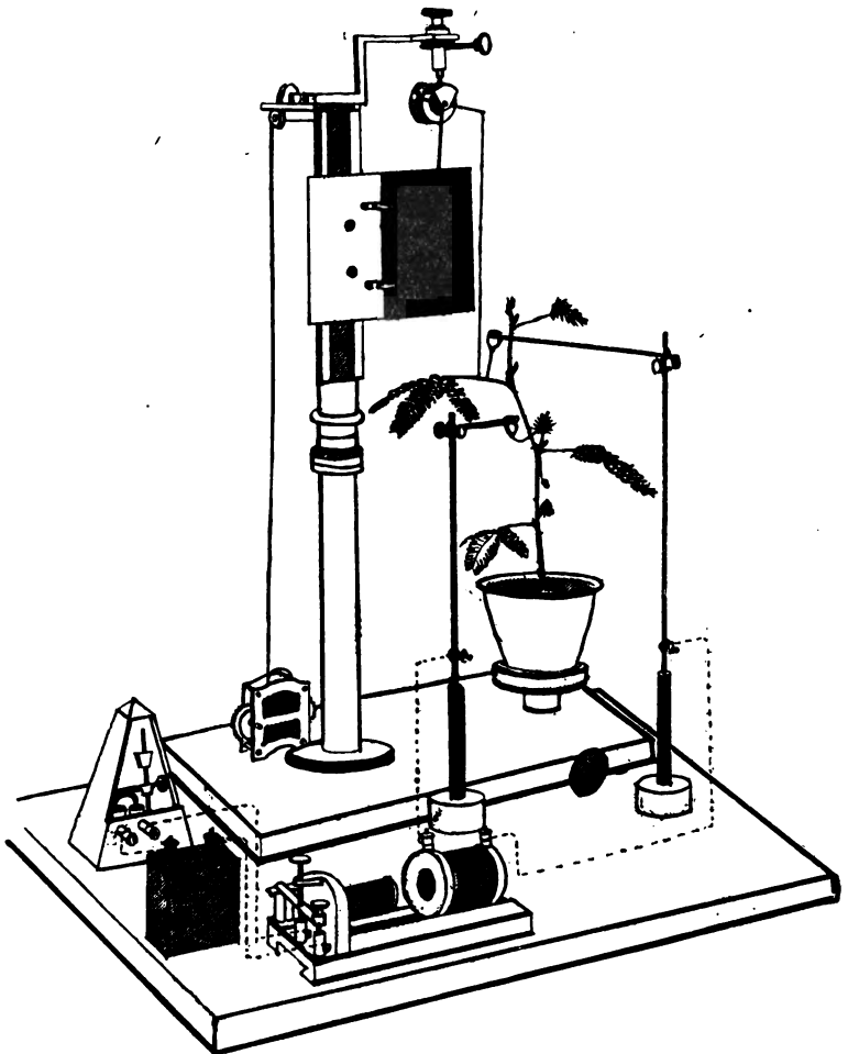
FIG. 11.—General view of the Resonant Recorder and the electrical connections by which excitatory shock of a definite duration is given to the plant; duration of shock determined by metronome, which completes electric circuit.
