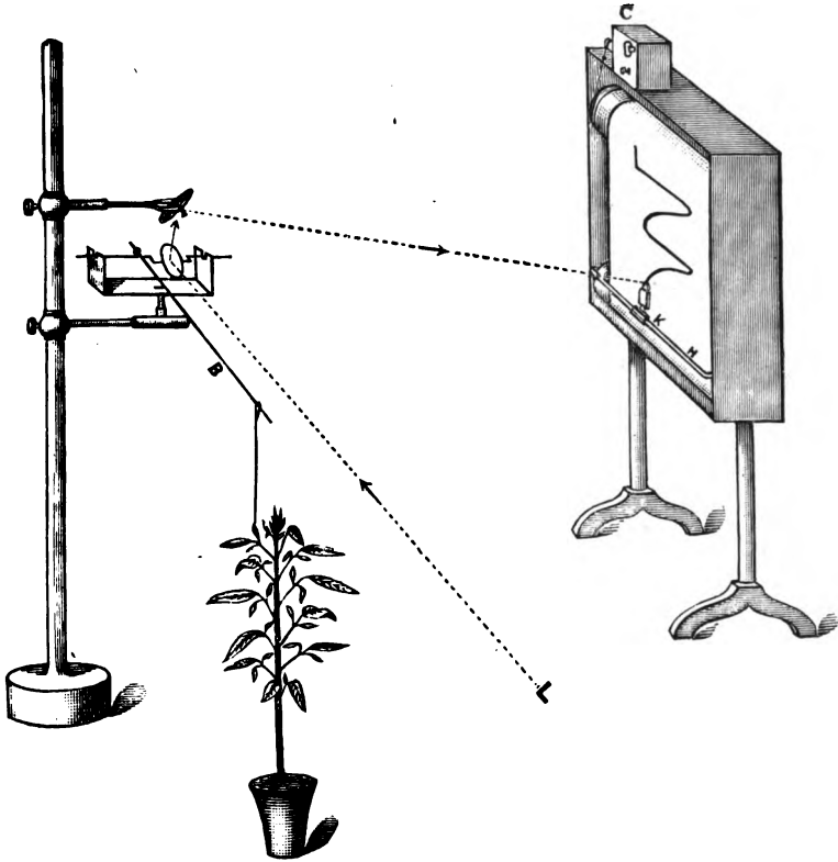
FIG. 7.—The Optical Pulse-Recorder. B, arm of optical lever attached to moving leaflet; L, ray of light, which after two reflections from the two mirrors falls on the recorder; C, clock-work, which keeps twin-drum—on which is wrapped the recording paper—revolving; H, horizontal guide bar; K, inkwell with projecting sponge.
