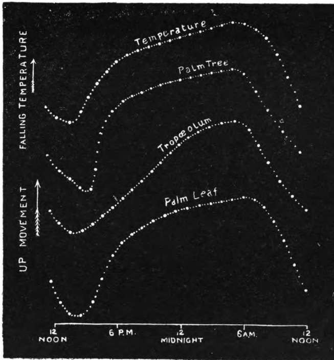
FIG. 25.—Records of the daily movement of the Palm Tree, of Tropaeolum , and of the Palm Leaf. The upper record gives the daily variation of temperature.
