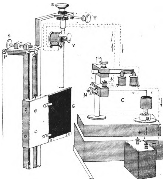
FIG. 10.—Upper part of the Resonant Recorder. Thread from clock, not shown, passes over pulley (P), letting down recording smoked glass plate (G); C, coercing reed which by its vibration sets recorder (V) in sympathetic vibration. The axis of recorder (V) is supported perpendicularly at centre of circular end of magnet. S S', adjusting screws; M, micrometer; T, tangent screw.
